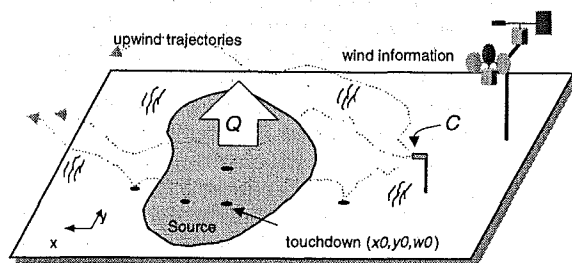
Figure 1: Illustration of bLS approach. Concentration C is measured downwind of the source, and Q is deduced from "touchdowns" inside the source.
