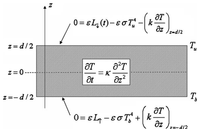
Fig. 1. Definitional schematic of idealized thermometric radiometer, and associated mathematical model.
